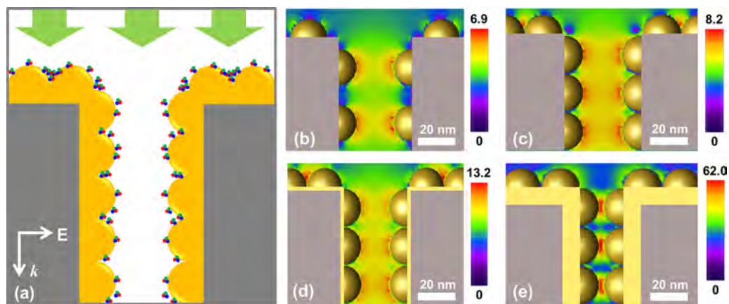
Fig. 5. The FDTD simulations for MnO 2 /Au hybrid nanowall film; (a) the model of MnO 2 /Au hybrid nanowall film for simulation; (b)–(e) FDTD simulations of the electric field distribution in cross-section view of MnO 2 /Au hybrid nanowall film with varied gold thickness.
