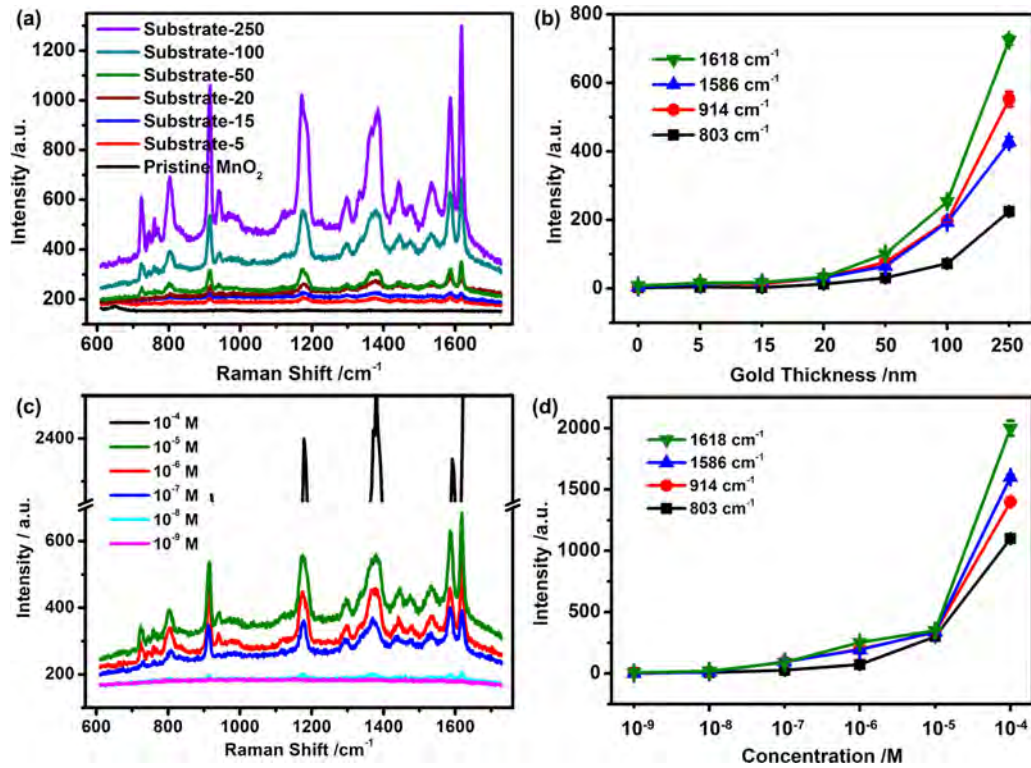
Fig. 4. (a) The raw Raman spectra of 1 \mu M CV on pristine MnO 2 nanowall, Substrate-5, Substrate-15, Substrate-20, Substrate-50, Substrate-100 and Substrate-250, respectively; (b) the Raman intensities of characteristic peaks with varied gold coating thickness; (c) the raw Raman spectra of different concentrations of CV ( 10^{-4} M, 10^{-5} M, 10^{-6} M, 10^{-7} M, 10^{-8} M, 10^{-9} M) on Substrate-100; (d) the Raman intensities of characteristic peaks with varied CV concentration.
