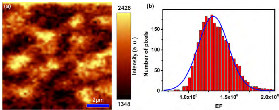
Fig. 7. (a) The Raman mapping of 1 μM CV on Substrate-200; (b) the histogram of EF distribution in mapping area.
