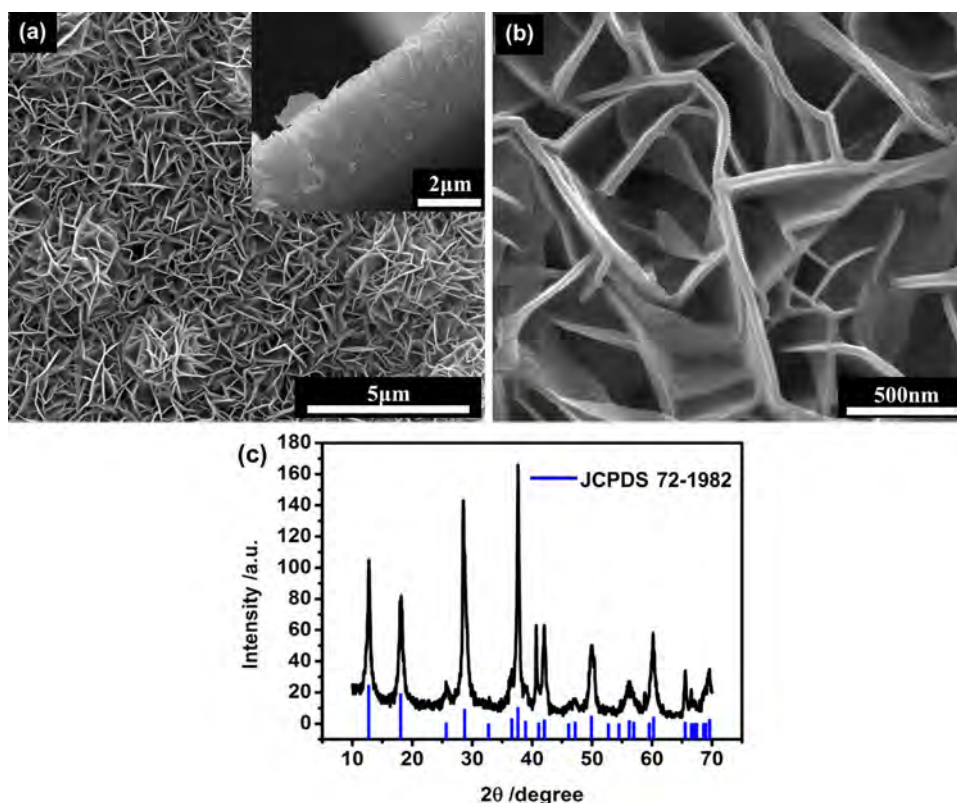
Fig. 2. (a) The top-view SEM image of MnO 2 nanowall film on silicon wafer, the inset is the cross-section view of the MnO 2 nanowall film; (b) the high magnification SEM image of the MnO 2 nanowall film; (c) the XRD pattern of the MnO 2 nanowall film.
